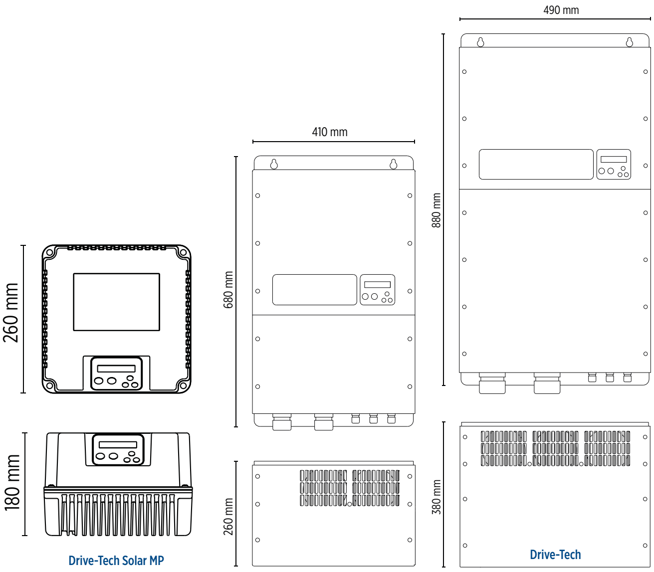
Drive-Tech COMPACT Solar MP
