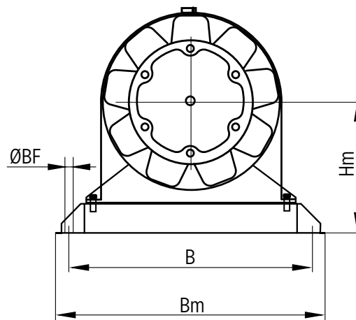
support flow sleeve / motor
