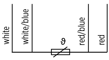
PT100 connection
