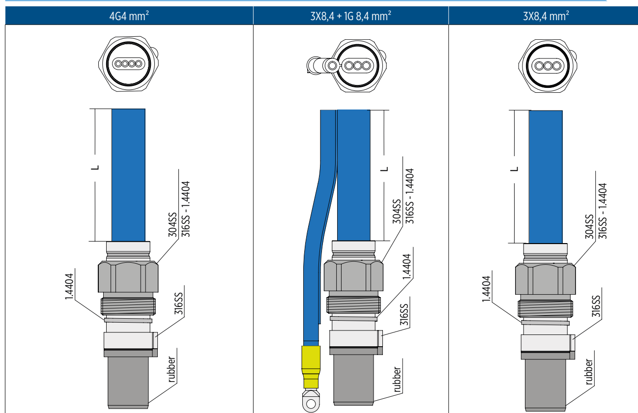
lead part numbers WW motors *
