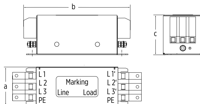
B84143A0080R106 (80 A)
